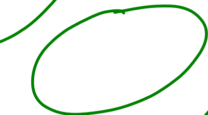
cyclic amide
