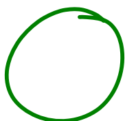
amine
